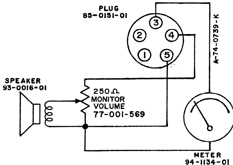
Model MMS-1 Monitor Speaker Panel, Schematic Diagram
